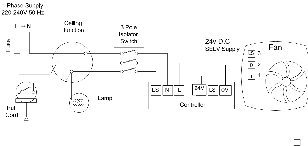
Fig.6 Continuous trickle with boost facility via LS or internal pullcord, ACR60LV model
