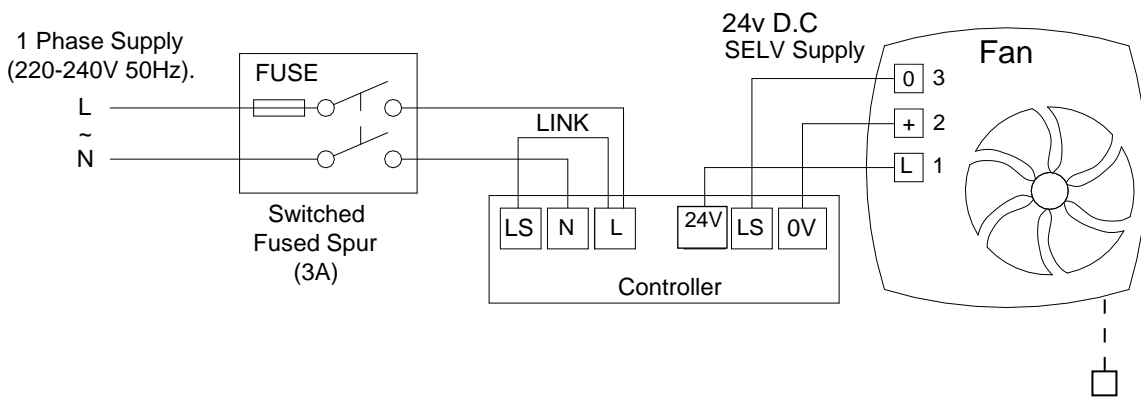
Fig.5 Continuous boost 1 with no trickle facility ACR60LV model
