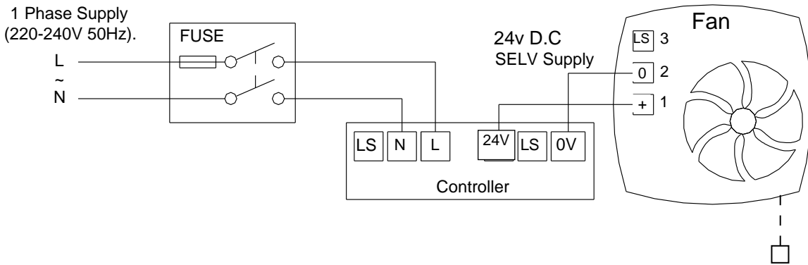
Fig.5 Continuous boost 1 with no trickle facility ACR60LV model
